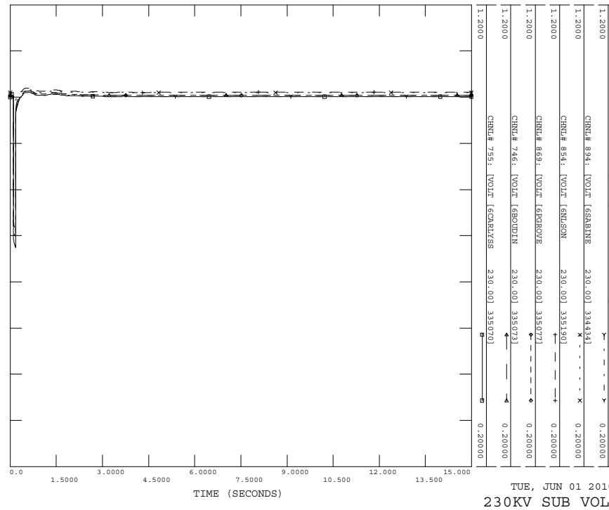
TUE, JUN 01 2010 14:14 DYNEGY MACHINE PLOTS
