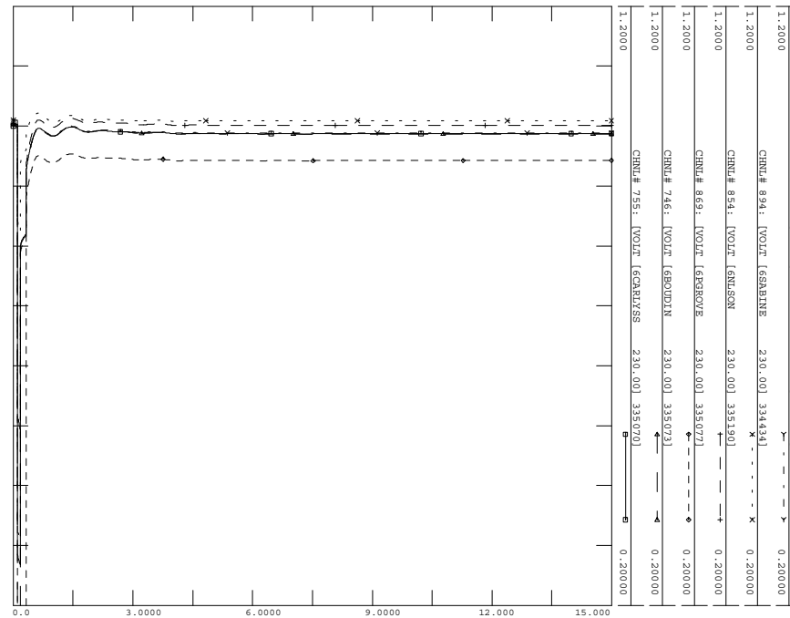
TUE, JUN 01 2010 14:13 230KV SUB VOLTAGES
