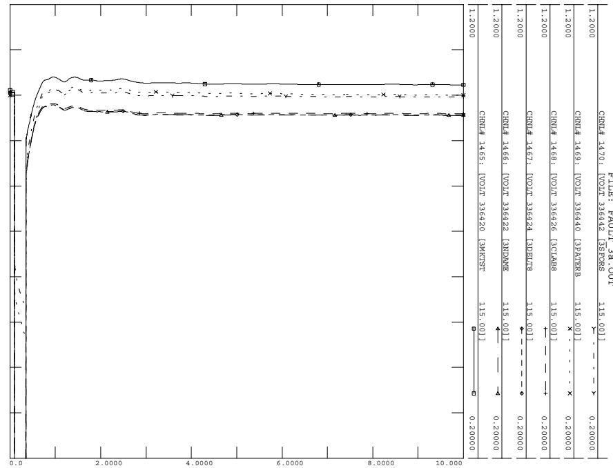
MON, MAY 25 2009 14:54 LOCAL AREA VOLTAGES
