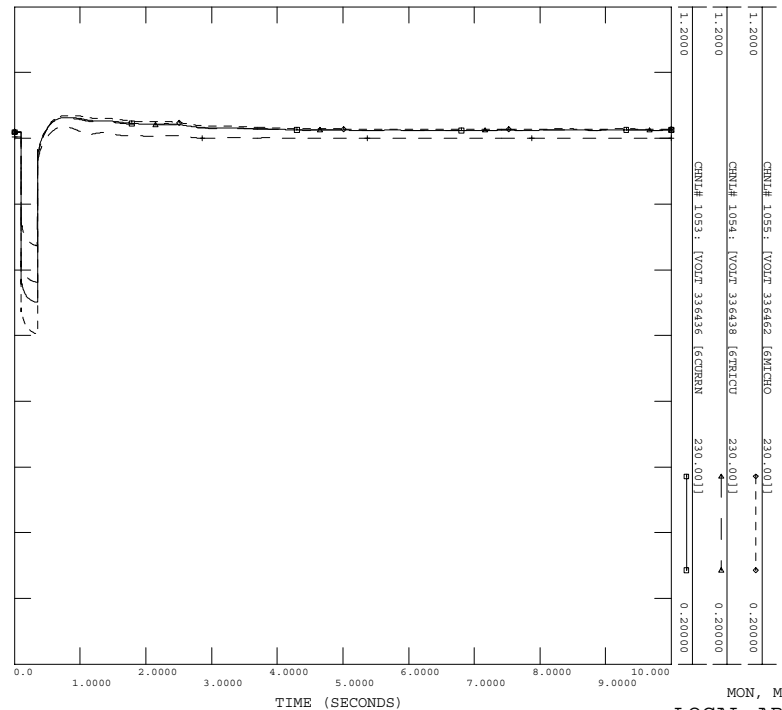
MON, MAY 25 2009 14:55 LOCAL AREA VOLTAGES
