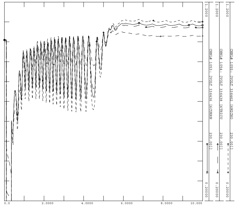
WED, JUN 10 2009 17:51 LOCAL AREA VOLTAGES
