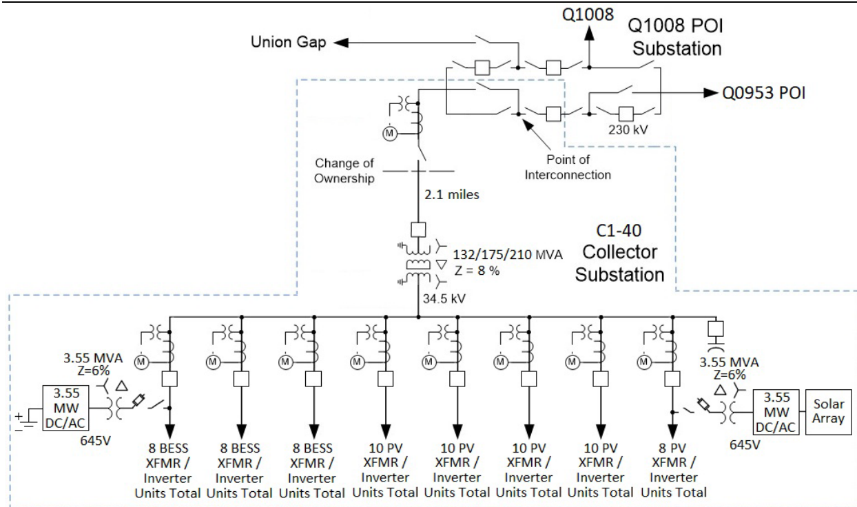
Figure 1: System One Line Diagram
