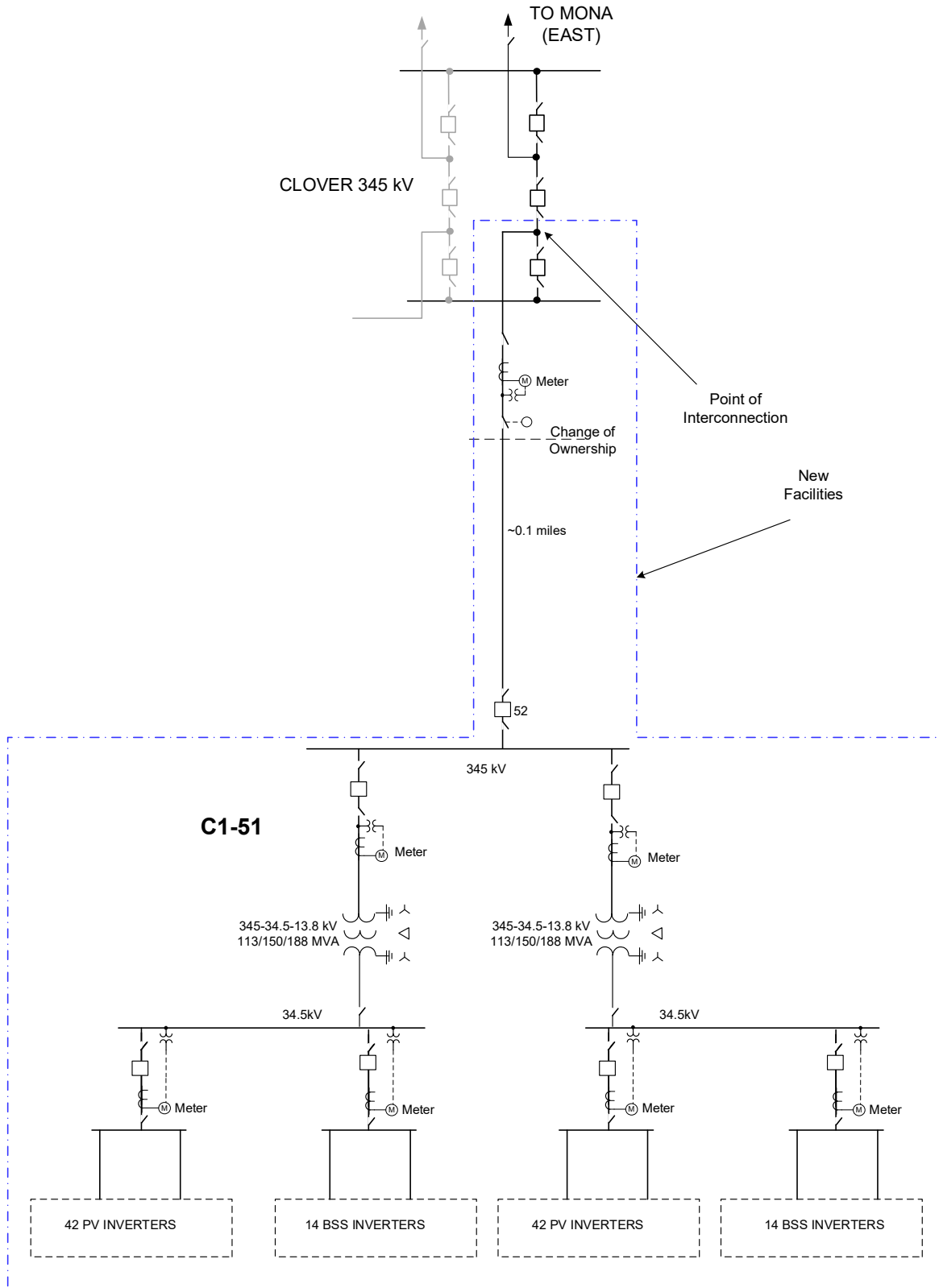
Figure 1: System One Line Diagram
