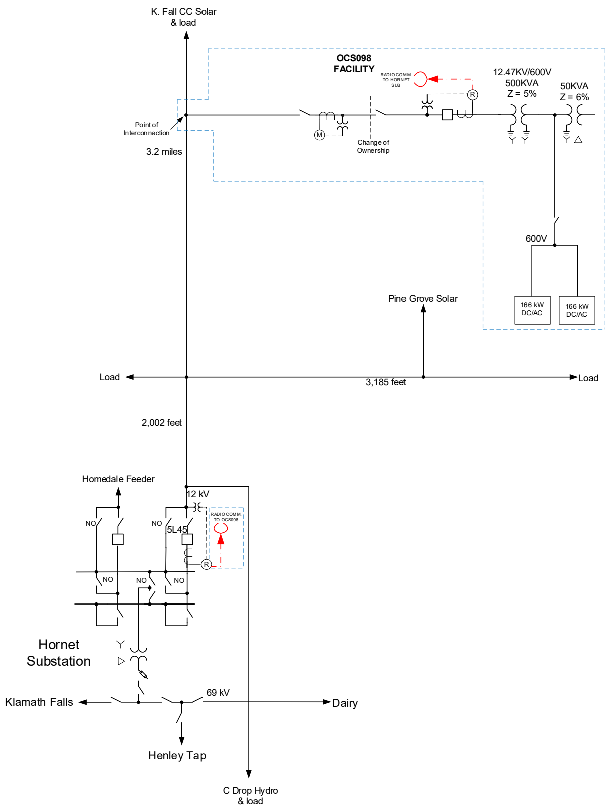
Figure 1: Feeder One Line Diagram
