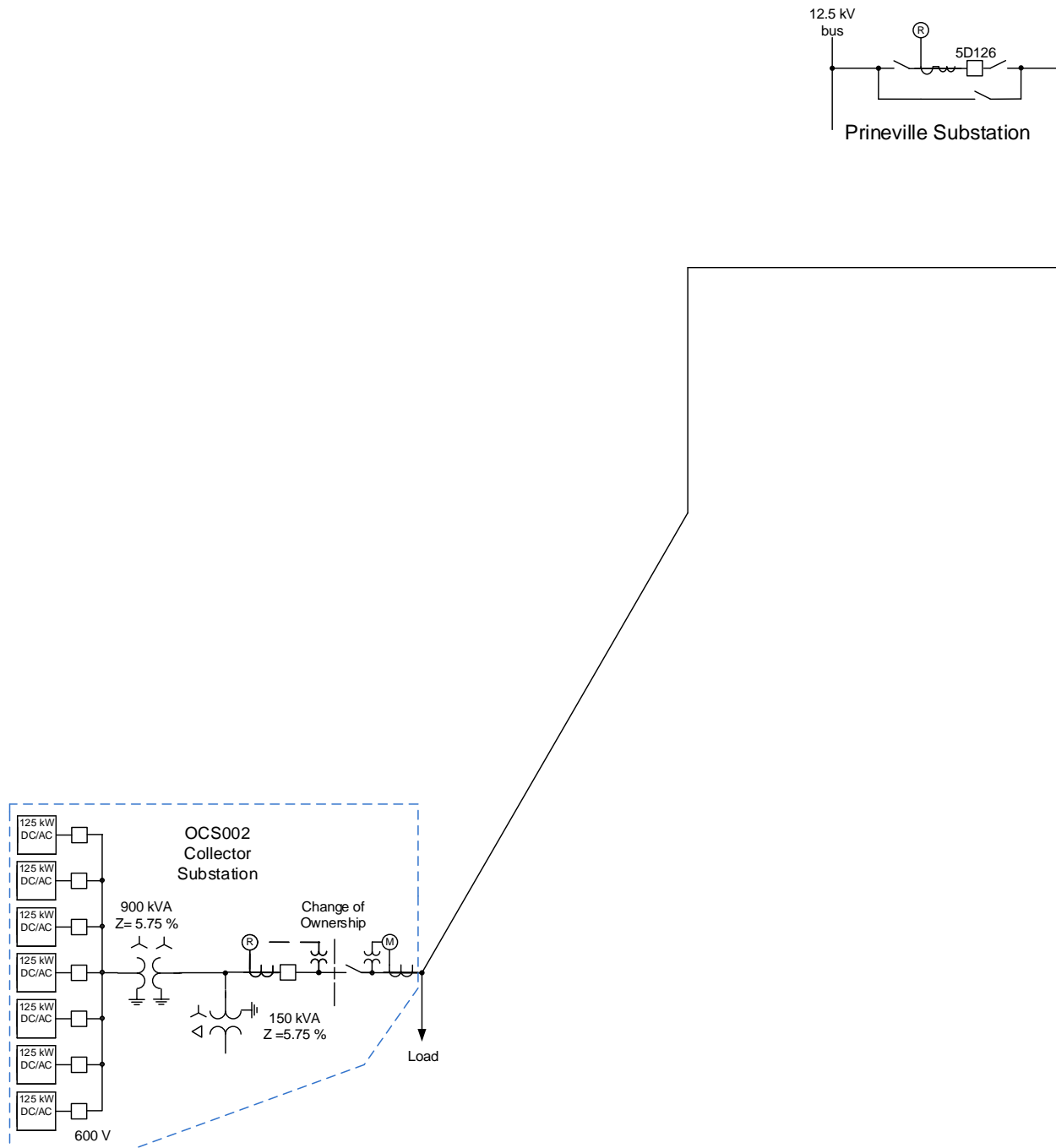
Figure 2: One Line Diagram
