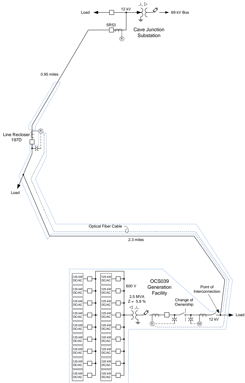
Figure 1: System One Line Diagram
