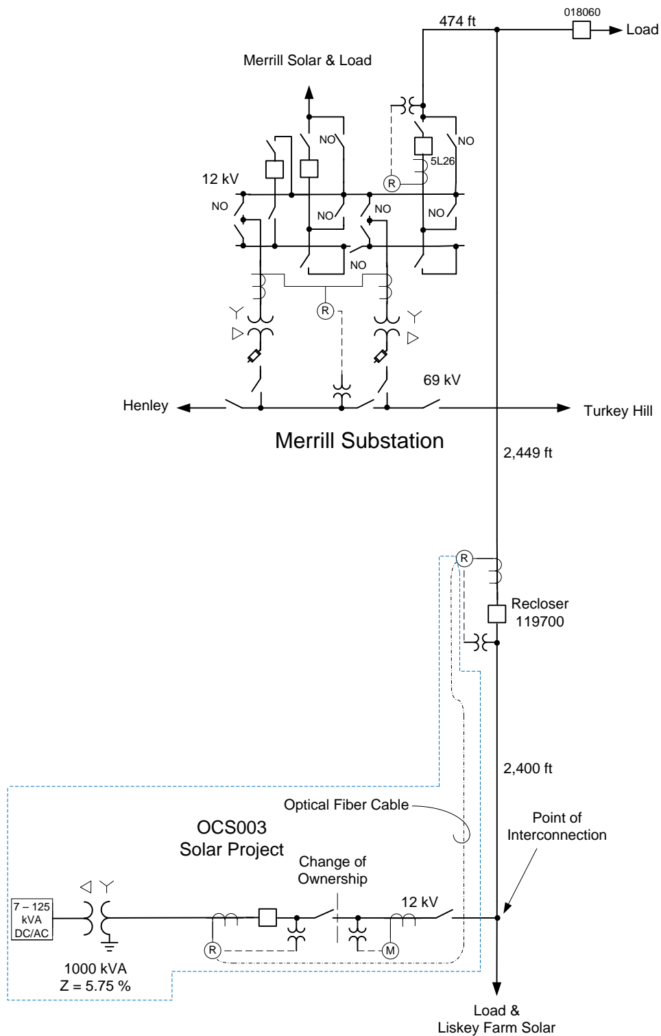
Figure 2: System One Line Diagram
