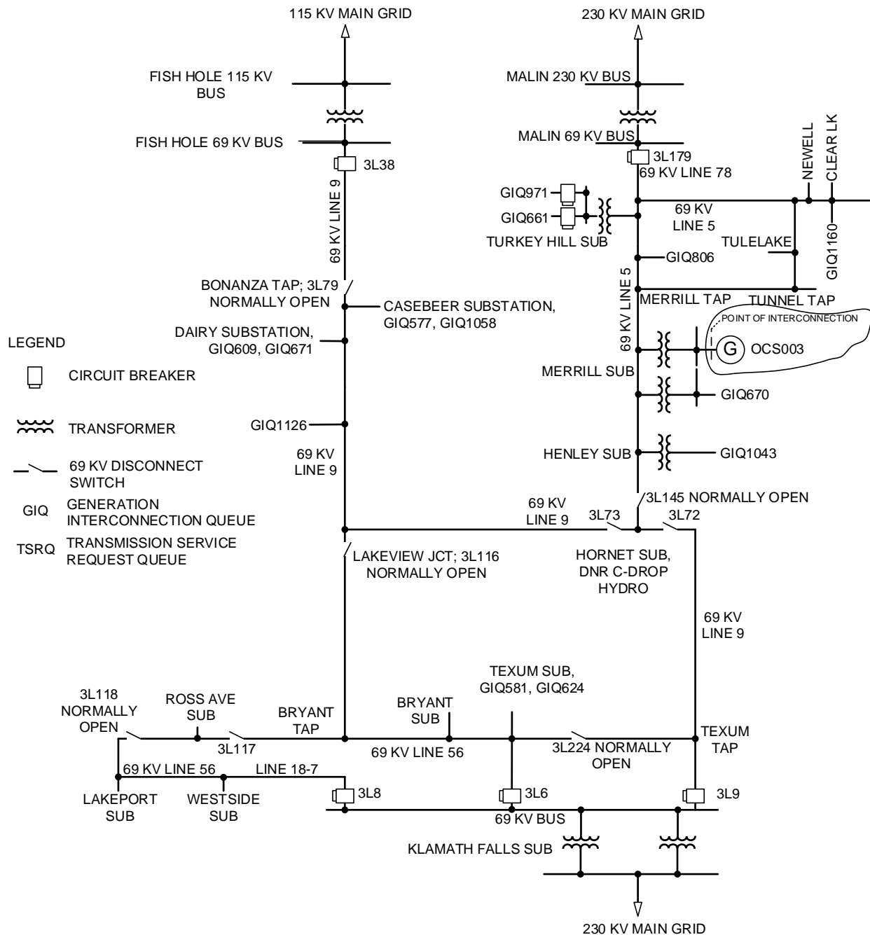
Figure 1: Transmission System One Line Diagram
