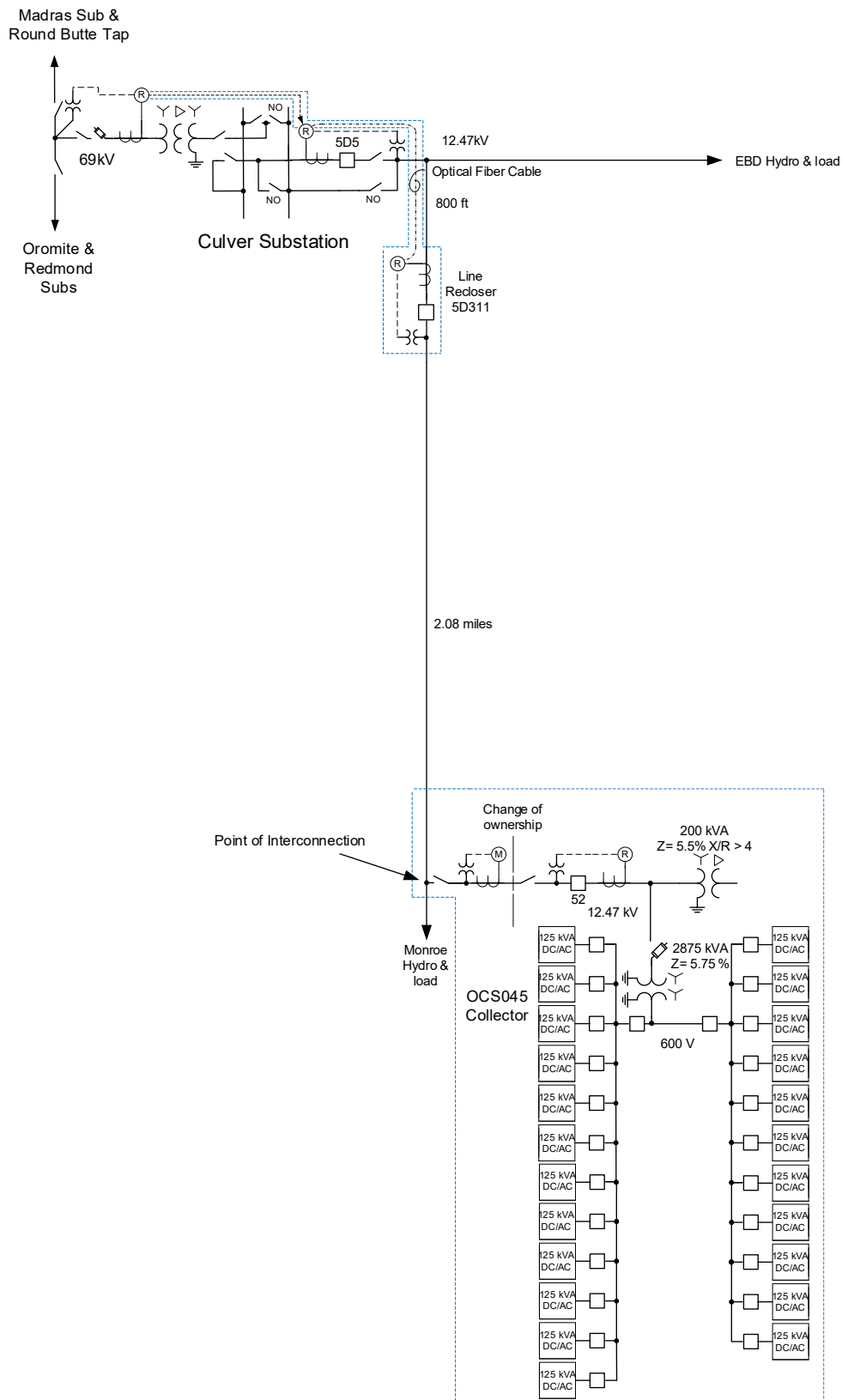
System One Line Diagram
