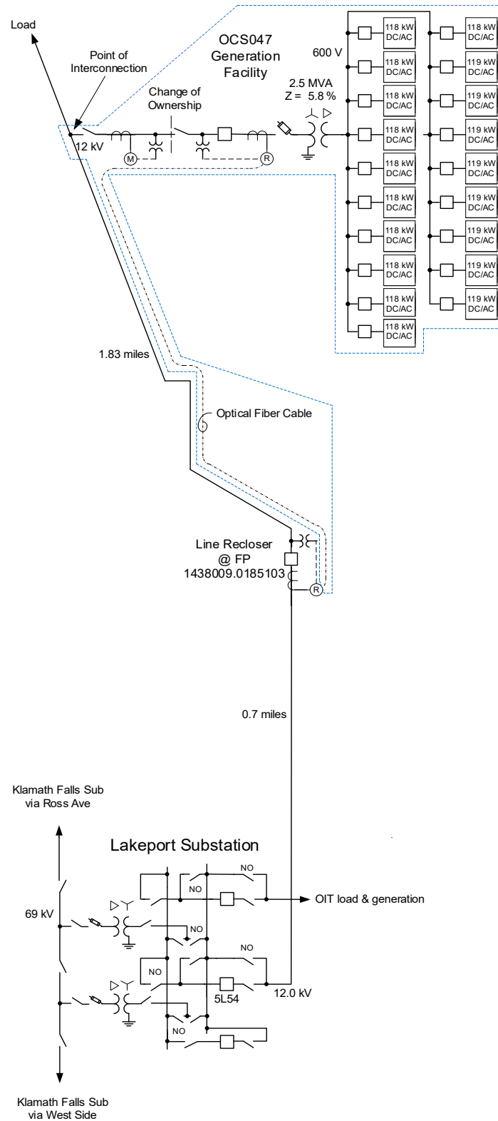
Figure 1: System One Line Diagram
