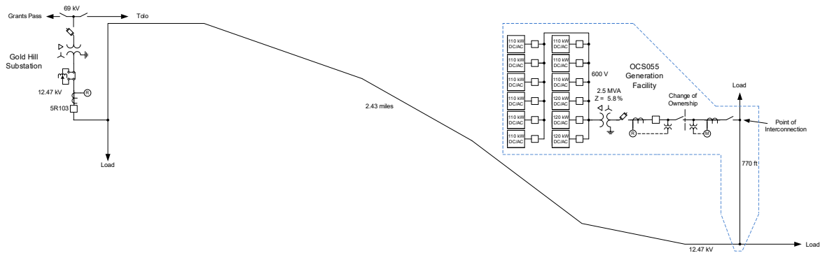
Figure 1: System One Line Diagram
