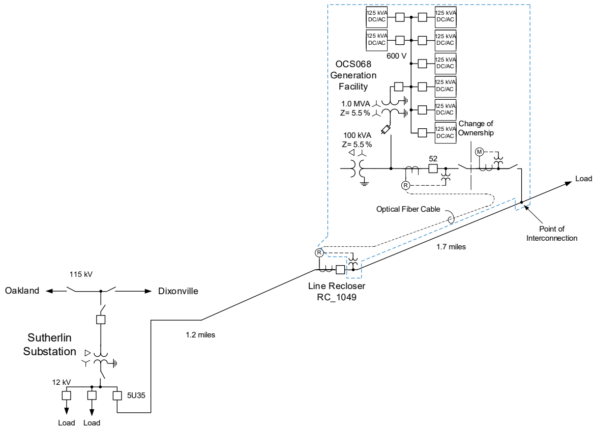
Figure 1: System One Line Diagram
