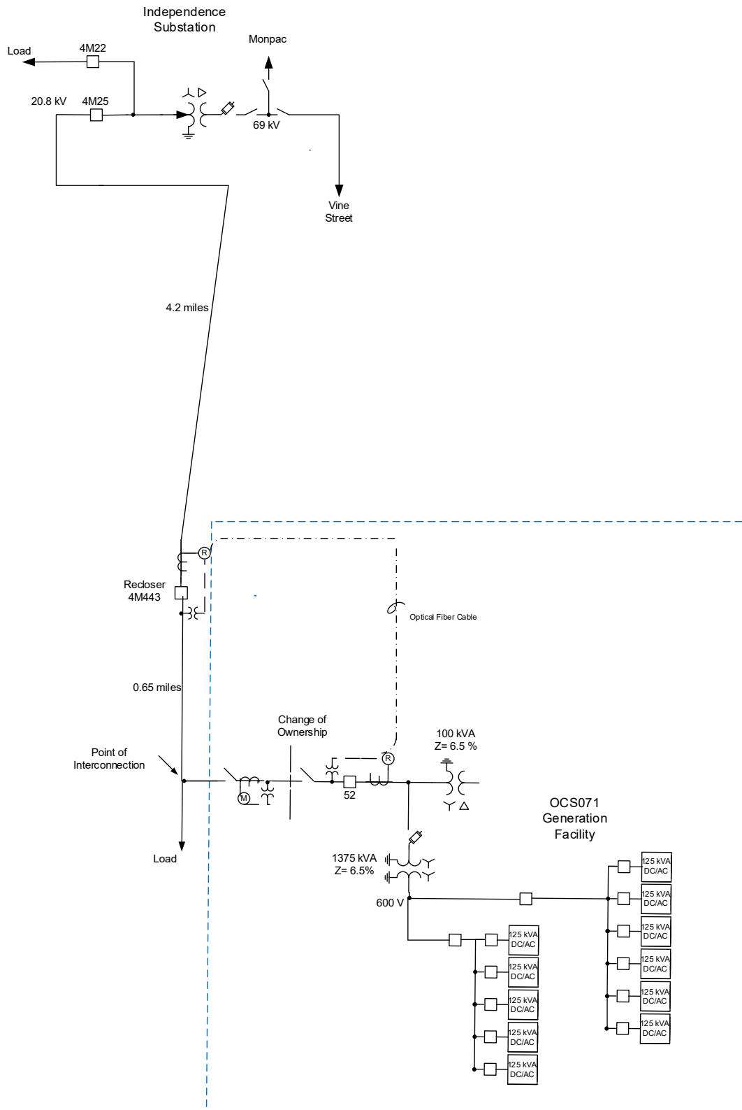
System One Line Diagram
