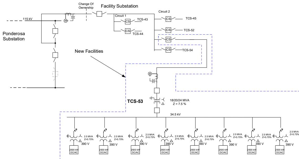
Figure 1: System One Line Diagram
