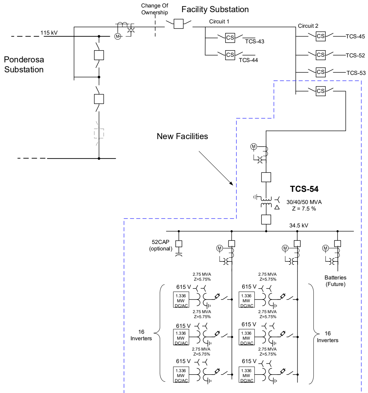
Figure 1: System One Line Diagram
